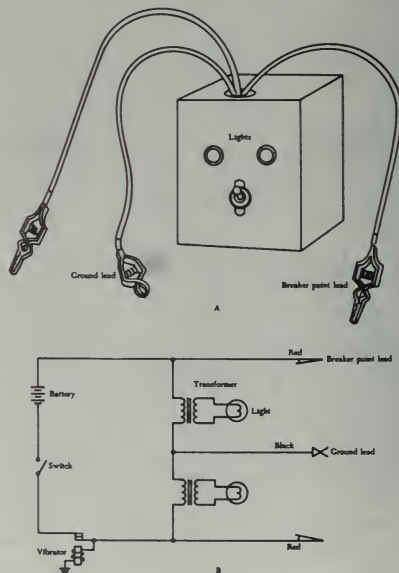
FIGURE 4-34. Timing light and wiring diagram.
